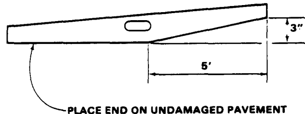
FIGURE A-3. FIVE PERCENT CHANGE OF SLOPE
